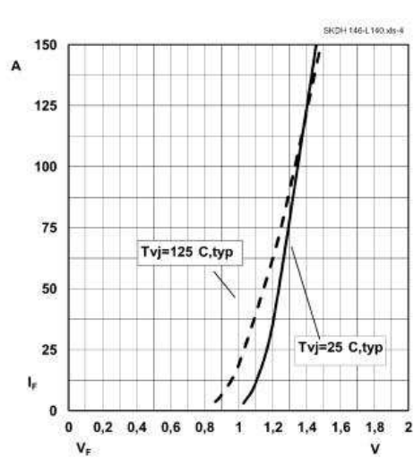
Fig. 4 Forward characteristic of single thyristor
